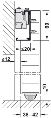
Floor Guide on Hard Floors
