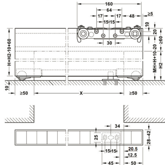
Floor Guide on Soft Floors with Running Track Provided on Site
