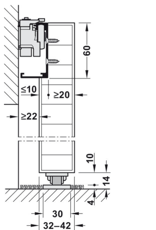
Floor Guide on Soft Floors with Running Track Provided on Site
