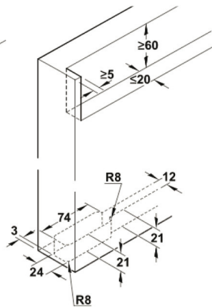
Concealed Installation
